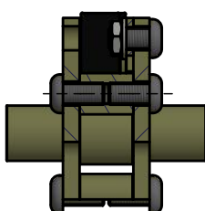
SECTION Z-Z
