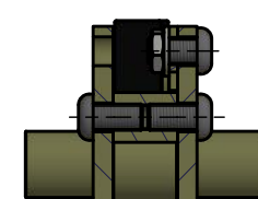
SECTION Z-Z
