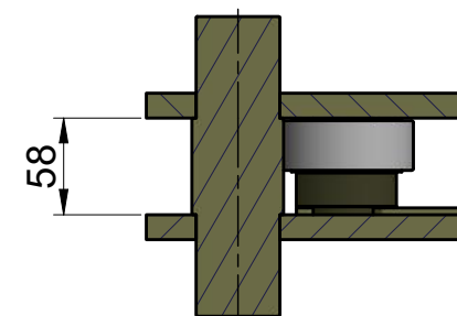
SECTION X-X
