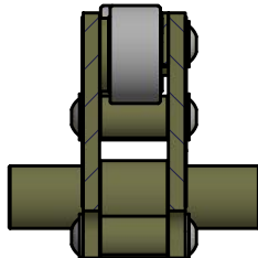
SECTION Y-Y
